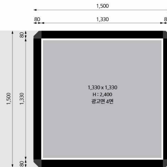
TOP VIEW SCALE : 1/10
